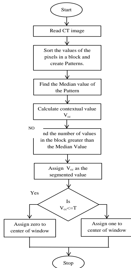
Fig. 2 Flow diagram of proposed algorithm
