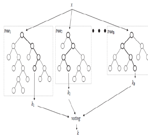
Fig. 3. Random Forest Classifier
